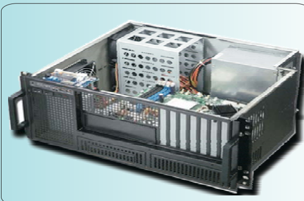
Inside View
